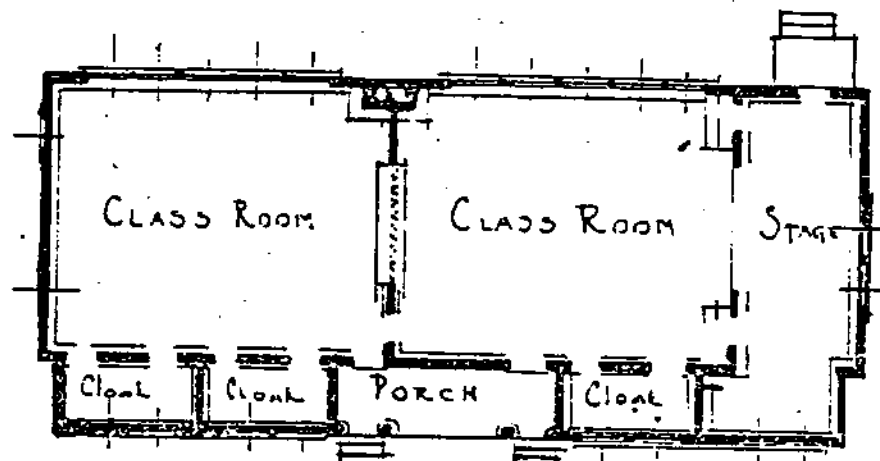
FLOOR PLAN
